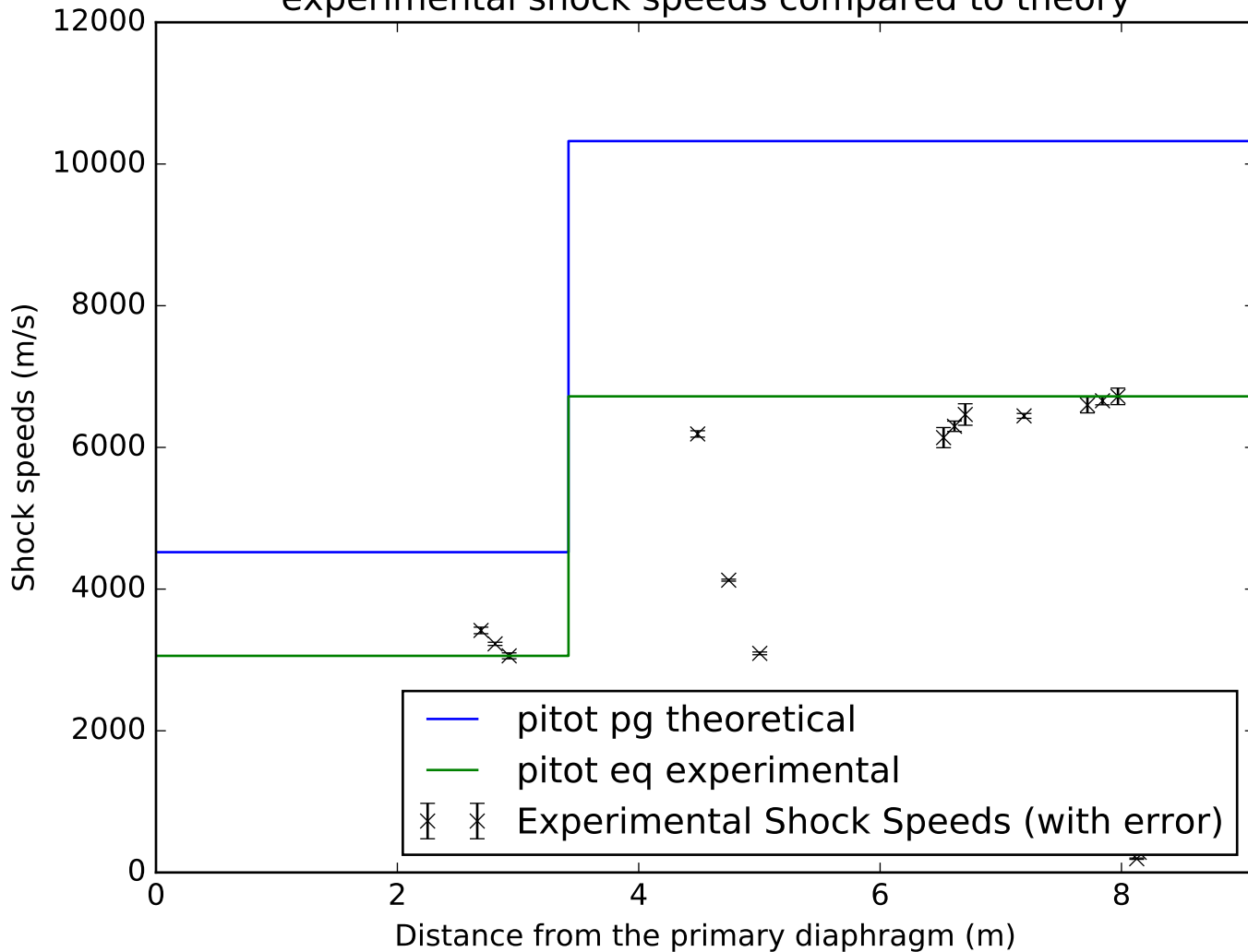
experimental shock speeds compared to theory
